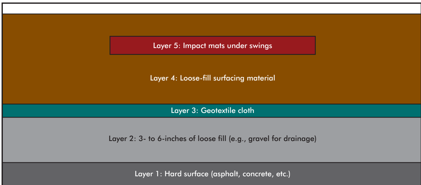
Figure 1. Installation layers for loose-fill over a hard surface
